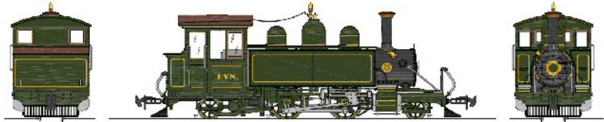
LYNTON & BAINSTAPLE RAILWAY - 18N BALDWIN 9-14 1-4-C (19) - DRAWING 11 CONSTR. NO. 15905 - 1898 BALDWIN STYLE - OLIVE GREEN & GOLD - STYLE 123
