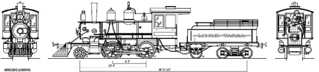
VICTORIAN POWELL WOOD PROCESS LTD BALDWIN 6-14-C (8) - LITTLE YARRA CONSTR. NO. 37718 - 1912
