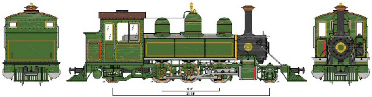
VICTORIAN RAILWAYS - V.A.1 BALDWIN 10-30 1-4-D (3) - DRAWING 1 CONSTR. NO. 15930 - 1898 BALDWIN STYLE - LIGHT IVY GREEN & GOLD - STYLE 202
